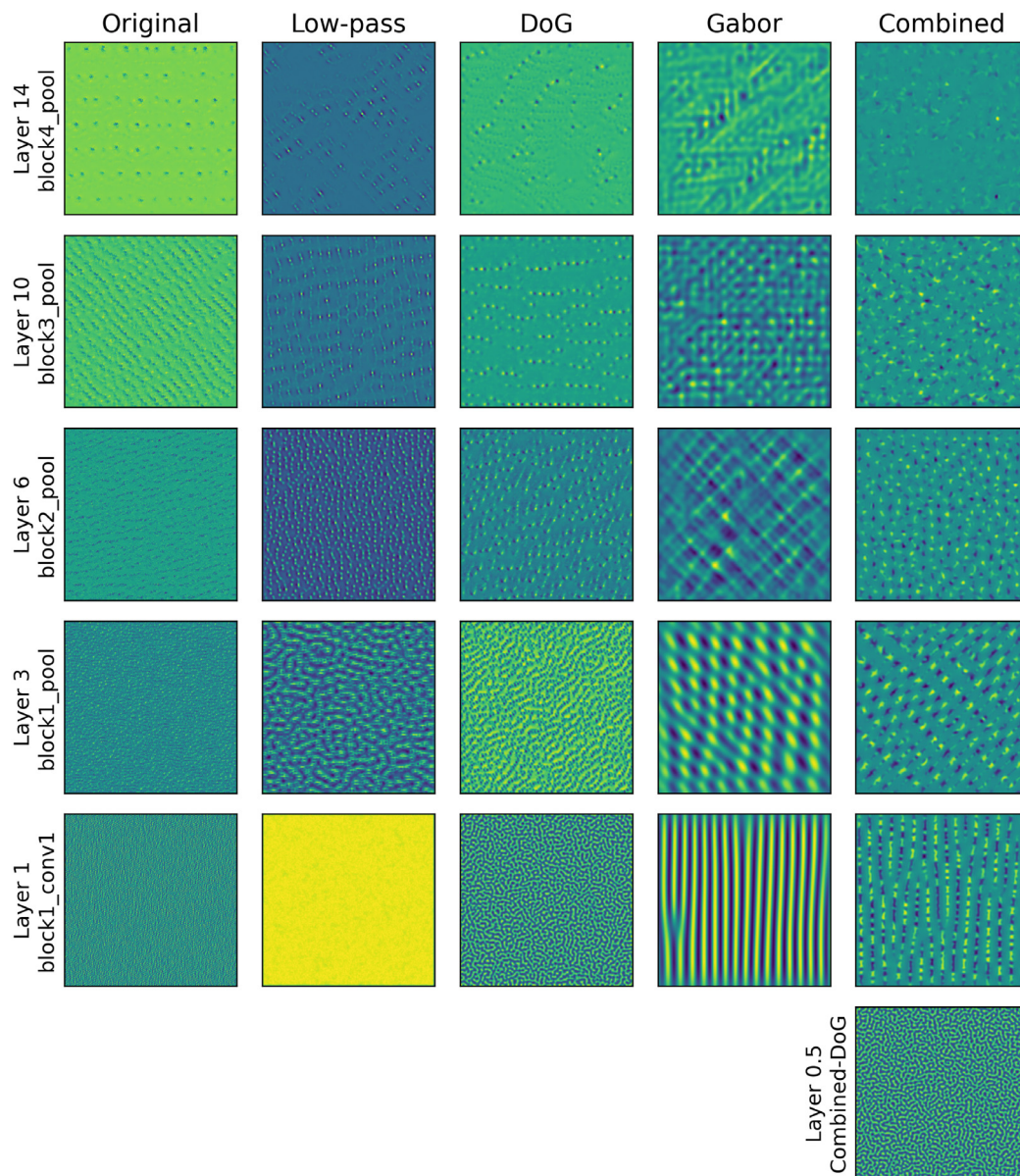
Fig. 10. Most activating features for a selection of layers in models based on VGG-16 with different initial convolutional layers.
