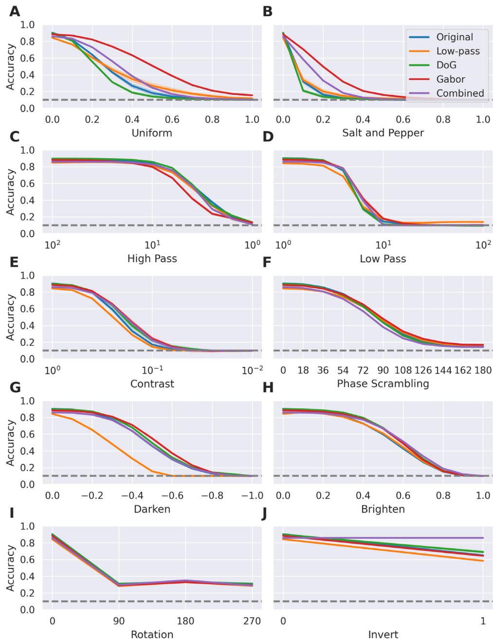
Fig. 6. Classification accuracy of VGG-16 based models under each type and degree of noise perturbation. The Gabor and Combined front-ends are particularly resilient to Uniform and Salt and Pepper noise, while the Combined front-end is able to recognise inverted images. Shading around each line indicates the 95% confidence interval across the five random seeds. The grey dashed lines represent chance level (10%) performance.
