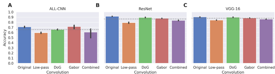
Fig. 5. Classification accuracy on the CIFAR-10 validation set. The ResNet and VGG models attained very similar levels of performance across all convolutional front-ends (around 90% accuracy) while ALL-CNN scored around 20% lower with more variability across front-ends. The line in each bar indicates the 95% confidence interval across the five random seeds. Grey dotted lines indicate the mean accuracy across convolutions for each base model architecture.
