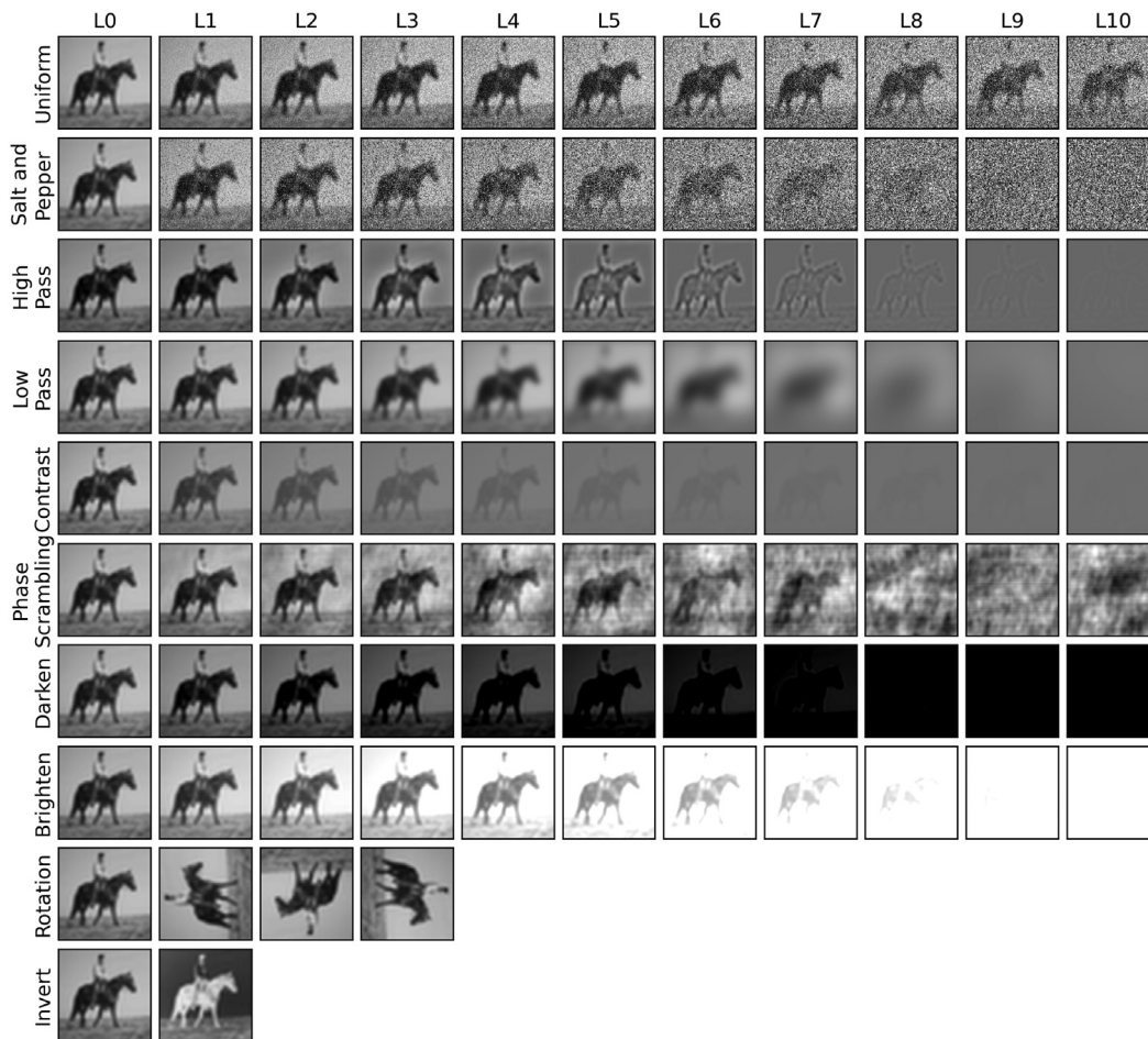
Fig. 2. Noise perturbations at each level applied to an example CIFAR-10 image.
