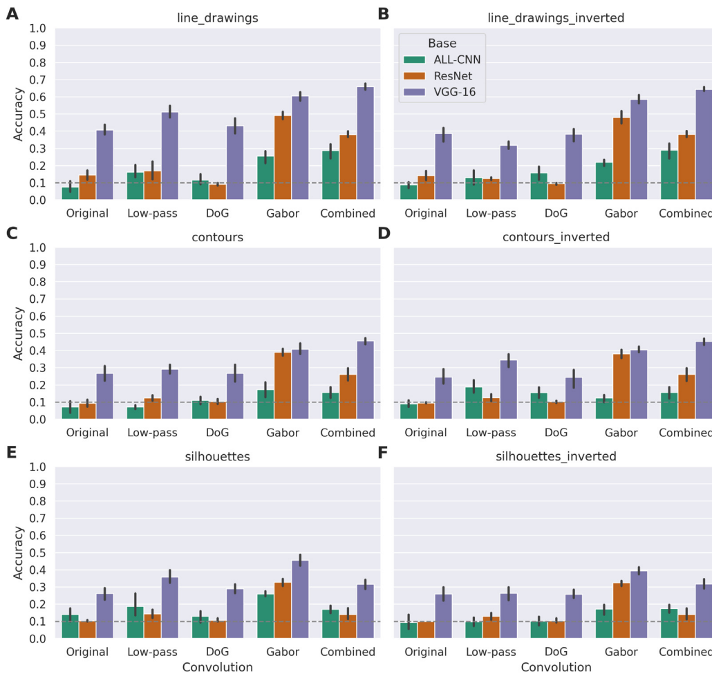
Fig. 7. Classification accuracy for generalisation test sets. In classifying out-of-distribution images, the Original (end-to-end) trained models typically score lowest. Classification accuracy with the Low-pass front end is slightly higher on average but less consistent across the test sets. The biologically-inspired convolutional front-ends have comparable performance (DoG front-ends) or substantially exceed the accuracy of the Original models (Gabor and Combined front-ends). Generally, all models score highest on the line drawings, with contours and silhouettes presenting the biggest challenges. The line in each bar indicates the 95% confidence interval across the five random seeds. The grey dashed lines represent chance level (10%) performance.
