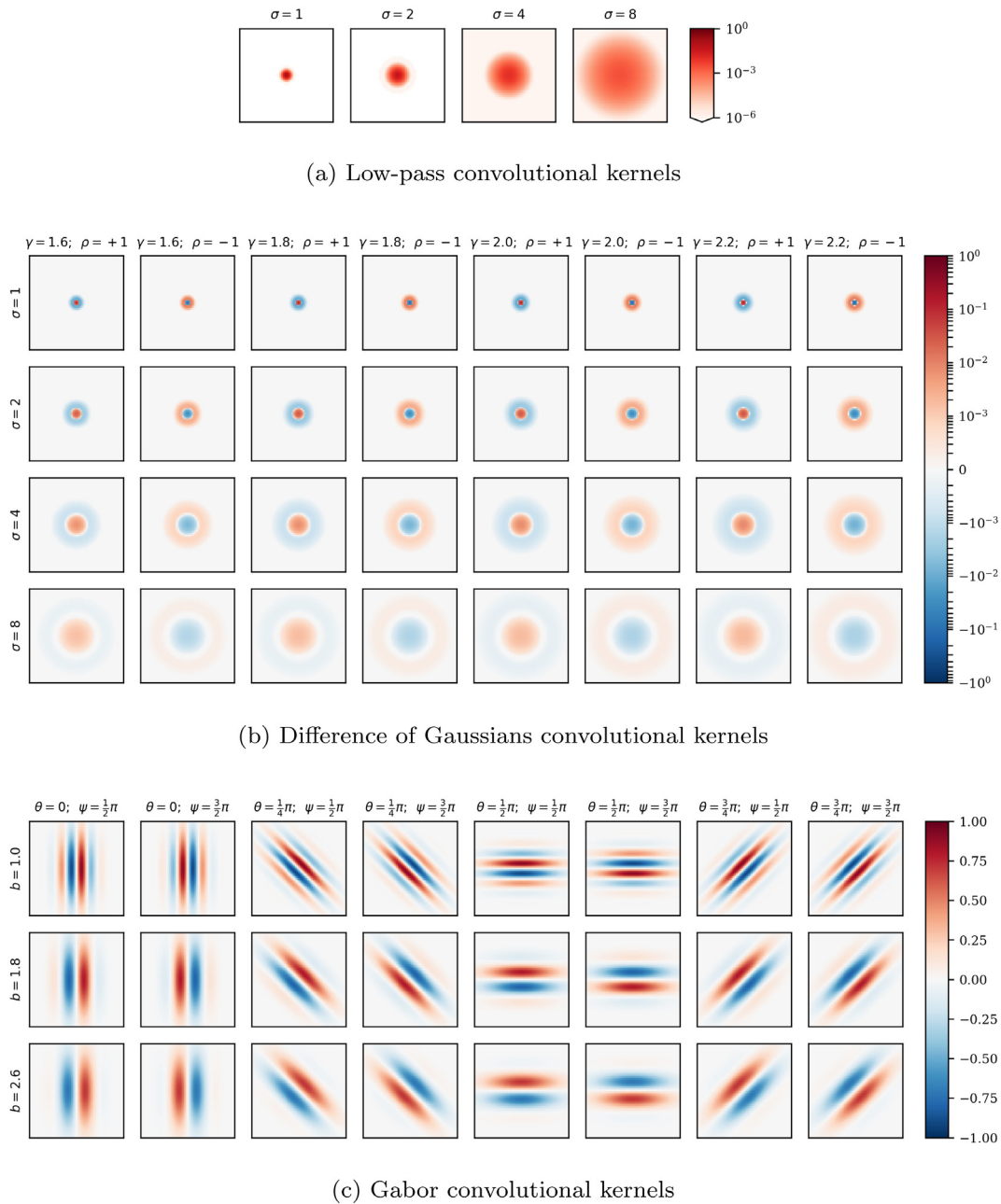
Fig. 1. Illustration of the banks of fixed kernels used in the first convolutional layer(s).
