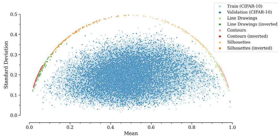
Fig. 4. Distributions of image statistics. The CIFAR-10 training and validation images are highly overlapping and occupy the central region of the space. Conversely, the generalisation images lie on a manifold forming an arc around this region, constituting out-of-distribution test sets.
