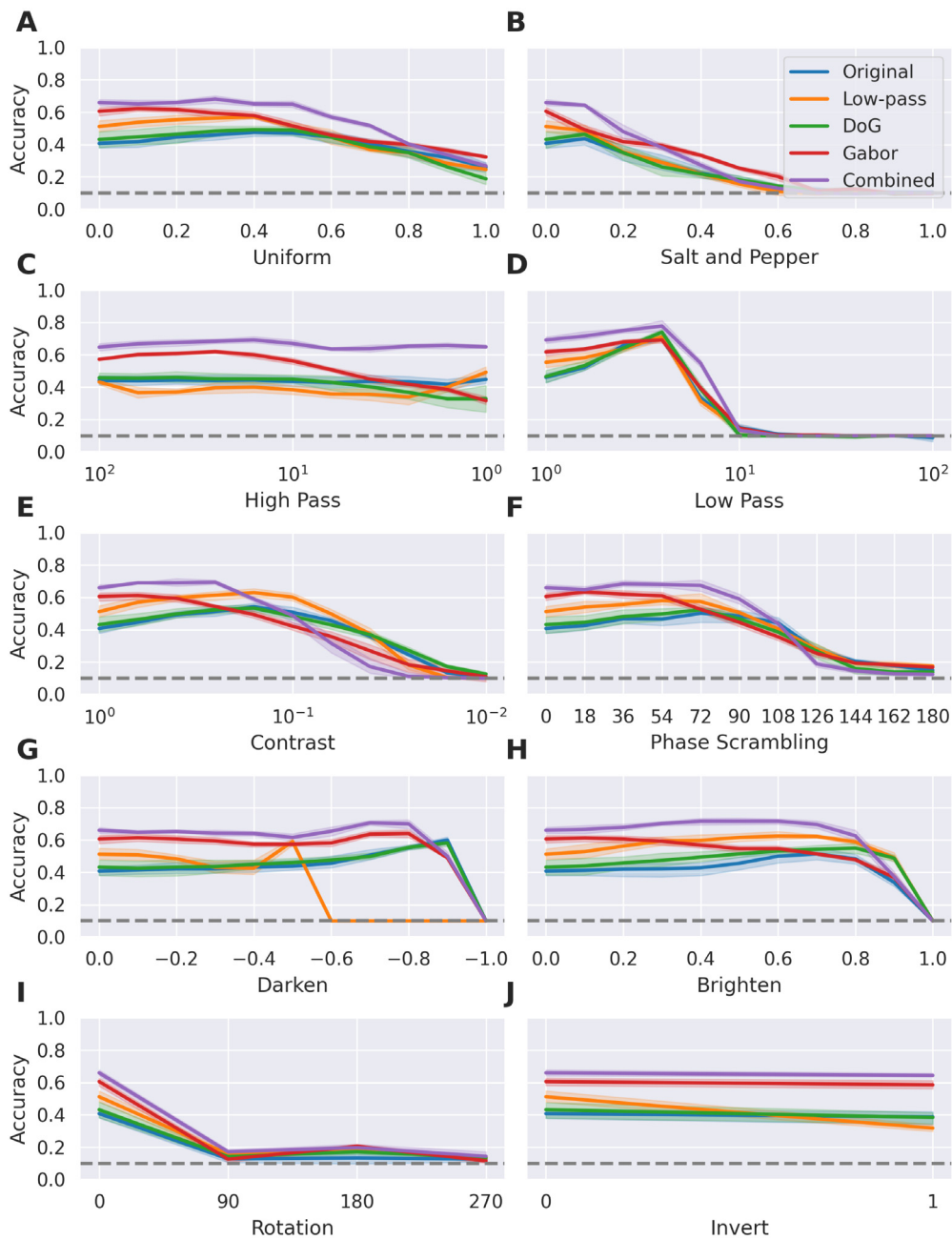
Fig. 9. Classification accuracy of VGG-16 based models on perturbed line drawings. The models with biologically-inspired convolutional front-ends (notably Gabor and Combined front-ends) typically maintain their advantage over the Original (end-to-end trained) models with the exception of low contrast and very dark perturbations. Shading around each line indicates the 95% confidence interval across the five random seeds. The grey dashed lines represent chance level (10%) performance.
